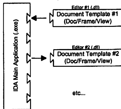
Figure 119 - IDA Main Application Architecture
